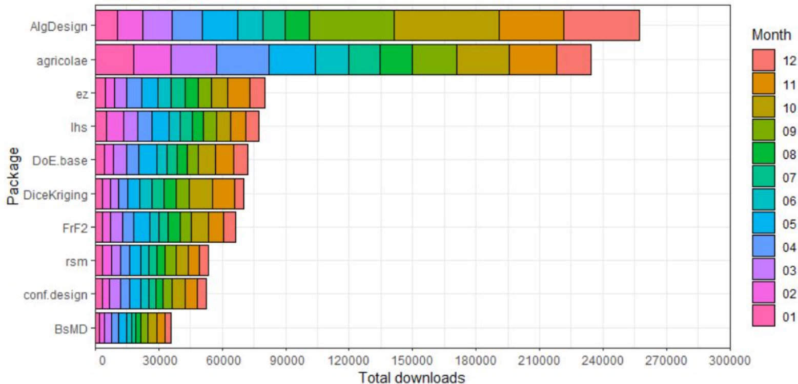
Top 10 R-packages for Design of Experiments (DoE)
